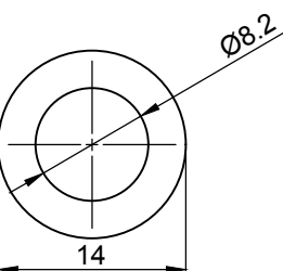
T=0.4 WASHER
